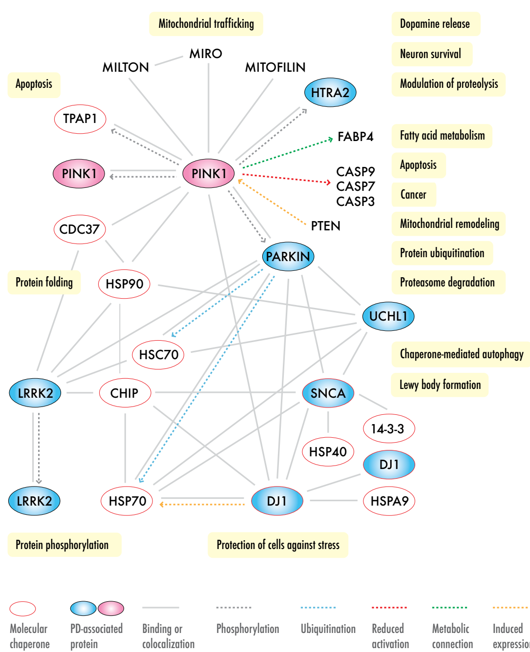
Fig. 5 Schematic representation of molecular interactions between PINK1, its functional partners and chaperones in Parkinson's disease. The biological processes, related to these protein interactions, are highlighted in yellow. CASP, caspase; MIRO, mitochondrial GTPase; PTEN, phosphatase and tensin homolog; Milton, adaptor protein; FABP4, fatty acid binding protein 4; Mitofilin, inner membrane protein, mitochondrial; 14-3-3, 14-3-3 protein beta/alpha; HSP40, DnaJ (Hsp40) homolog, subfamily 8, member 6 (8).
