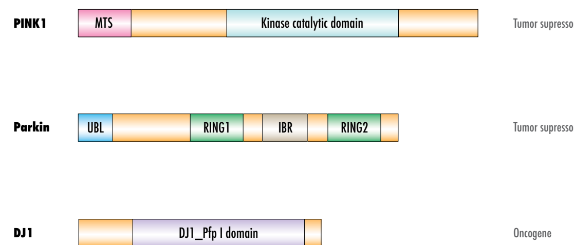
Fig. 4 Domain architecture of PINK1, Parkin and DJ1 proteins. In PD, these autosomal recessive genes are linked to oxidative stress or mitochondrial dysfunction. MTS, mitochondrial targeting sequence; UBL, ubiquitin-like domain; RING, RING finger motif; IBR, in between ring fingers (4).
