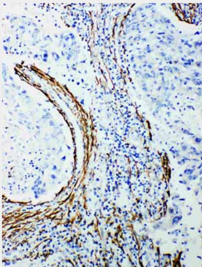
Anti-Ataxin 3 antibody, ABO11154, IHC(P) IHC(P): Human Lung Cancer Tissue
