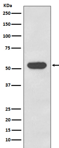
Western blot analysis of Cytokeratin 4 expression in A431 cell lysate.
