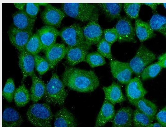
Figure 2. IF analysis of CCT3 using anti-CCT3 antibody (M05920).
