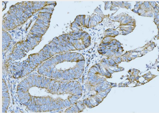
Figure 4. IHC analysis of Cytokeratin 5 using anti-Cytokeratin 5 antibody (M00398-7). Cytokeratin 5 was detected in a paraffin-embedded section of human rectal moderately differentiated adenocarcinoma tissue. Heat mediated antigen retrieval was performed in EDTA buffer (pH 8.0, epitope retrieval solution). The tissue section was blocked with 10% goat serum. The tissue section was then incubated with 2 µg/ml mouse anti-Cytokeratin 5 Antibody (M00398-7) overnight at 4°C. Biotinylated goat anti-mouse IgG was used as secondary antibody and incubated for 30 minutes at 37°C. The tissue section was developed using Streptavidin-Biotin-Complex (SABC) (Catalog # SA1021) with DAB as the chromogen.
