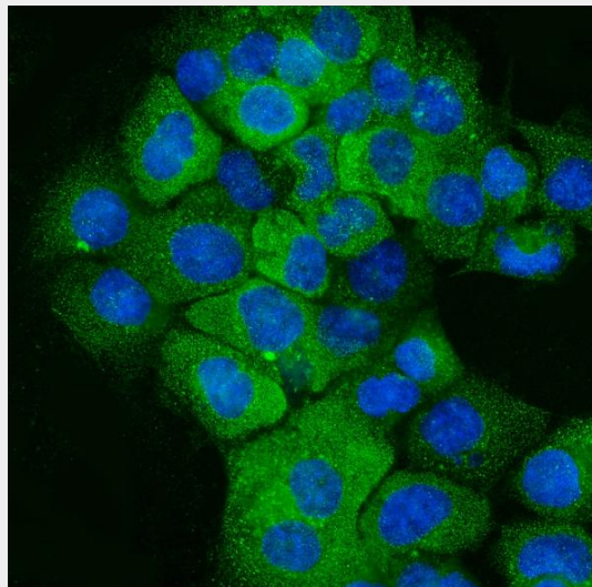
Figure 5. IF analysis of Cytokeratin 5 using anti-Cytokeratin 5 antibody (M00398-7). Cytokeratin 5 was detected in an immunocytochemical section of A431 cells. Enzyme antigen retrieval was performed using IHC enzyme antigen retrieval reagent (AR0022) for 15 mins. The cells were blocked with 10% goat serum. And then incubated with 5 µg/mL mouse anti-Cytokeratin 5 Antibody (M00398-7) overnight at 4°C. DyLight®488 Conjugated Goat Anti-Mouse IgG (BA1126) was used as secondary antibody at 1:100 dilution and incubated for 30 minutes at 37°C. The section was counterstained with DAPI. Visualize using a fluorescence microscope and filter sets appropriate for the label used.
