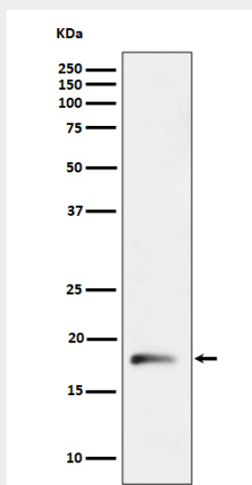
Western blot analysis of RPL26L1 expression in HepG2 cell lysate.
