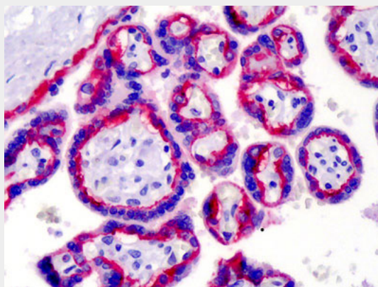
Anti-Integrin Beta 4 antibody IHC of human placenta.
