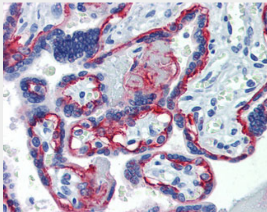
Anti-Integrin Beta 4 antibody IHC of human placenta.
