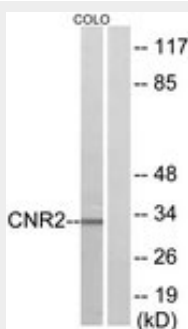
Western blot of extracts from COLO205 cells, using CNR2 Antibody.
