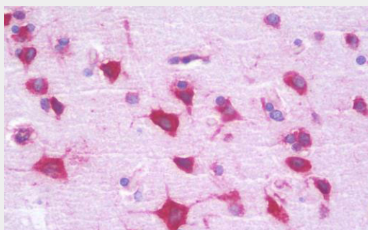
Anti-RPL35 antibody IHC staining of human brain, cortex.
