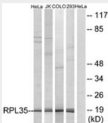
Western blot of extracts from 293/HeLa/COLO/Jurkat cells, using RPL35 Antibody.
