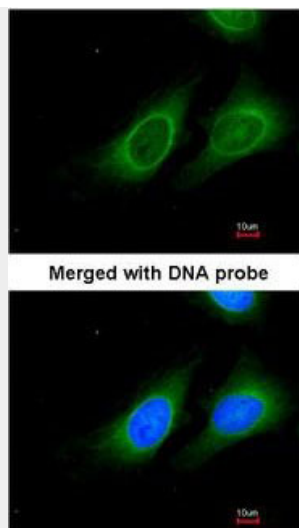
Immunofluorescence of paraformaldehyde-fixed HeLa using 15-PGDH antibody at 1:200 dilution.
