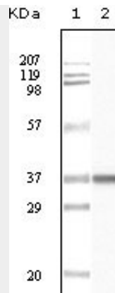
Figure 1: Western blot analysis using BLK mouse mAb against truncated BLK recombinant protein.
