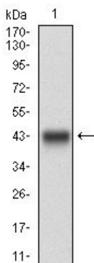
Figure 1: Western blot analysis using DNM1L mAb against human DNM1L recombinant protein. (Expected MW is 41.8 kDa)
