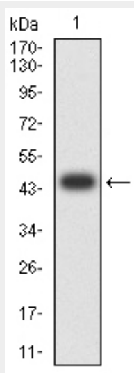
Figure 2: Western blot analysis using ATRX mAb against human ATRX (AA: 2311-2492) recombinant protein. (Expected MW is 46.6 kDa)
