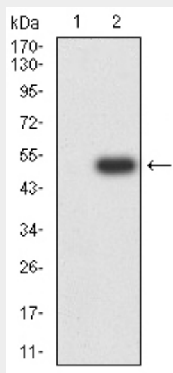
Figure 3: Western blot analysis using ATRX mAb against HEK293 (1) and ATRX (AA: 2311-2492)-hlgGfc transfected HEK293 (2) cell lysate.
