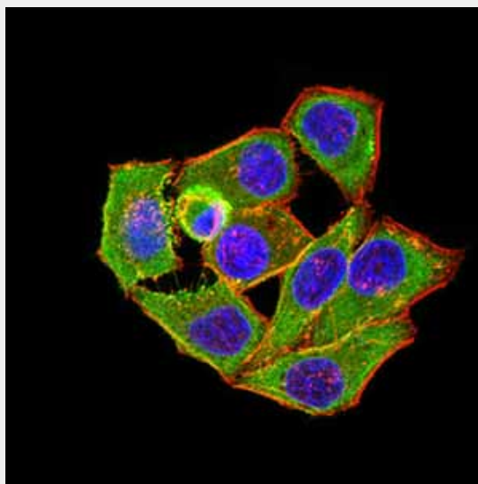
Figure 4: Immunofluorescence analysis of HeLa cells using ANAPC1 mouse mAb (green). Blue: DRAQ5 fluorescent DNA dye. Red: Actin filaments have been labeled with Alexa Fluor- 555 phalloidin. Secondary antibody from Fisher (Cat#: 35503)
