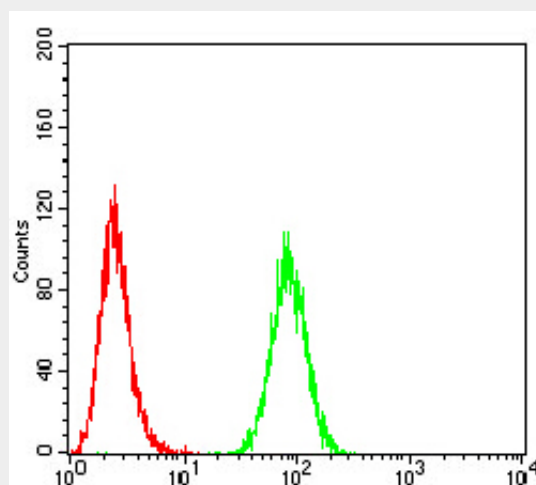
Figure 5: Flow cytometric analysis of HeLa cells using ANAPC1 mouse mAb (green) and negative
