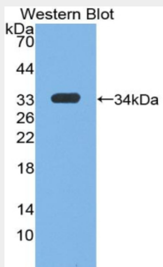
Figure. Western Blot; Sample: Recombinant IGF1, Porcine.
