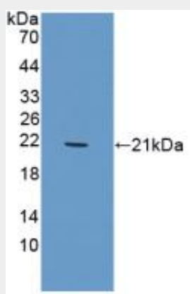
Figure. Western Blot; Sample: Recombinant TREM1, Porcine.
