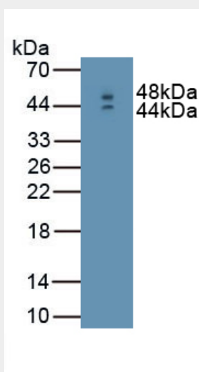
Figure. Western Blot; Sample: Recombinant IFNb, Mouse.
