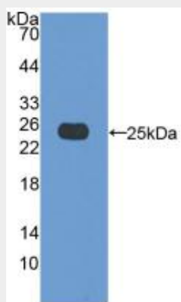
Figure. Western Blot; Sample: Recombinant Bax, Porcine.
