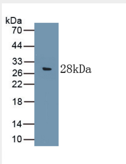
Figure. Western Blot; Sample: Recombinant C9, Rat.
