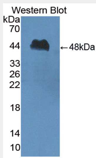
Figure. Western Blot; Sample: Recombinant PI16, Bovine.
