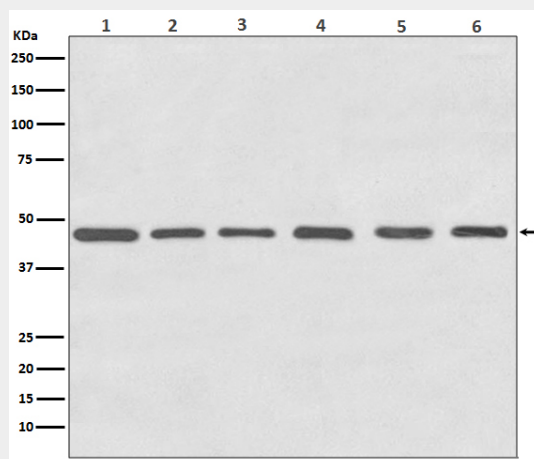
Western blot analysis of Tubulin gamma expression in (1) HeLa cell lysate; (2) NIH 3T3 cell lysate; (3) C6 cell lysate; (4) Zebrafish lysates; (5) COS-1 cell lysate; (6) MDCK cell lysate.
