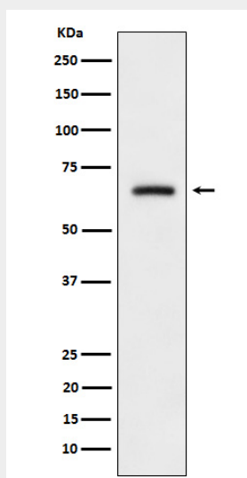
Western blot analysis of CRMP3 expression in SH-SY5Y cell lysate.
