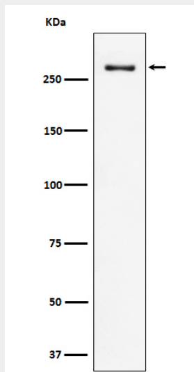
Western blot analysis of CHD3 expression in HeLa cell lysate.
