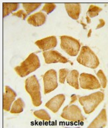
Formalin-fixed and paraffin-embedded human skeletal muscle reacted with ANP32A Antibody (C-term), which was peroxidase-conjugated to the secondary antibody, followed by DAB staining. This data demonstrates the use of this antibody for immunohistochemistry; clinical relevance has not been evaluated.
