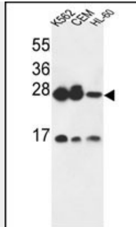
ANP32A Antibody (C-term) (Cat. #AP9520b) western blot analysis in K562,CEM,HL-60 cell line lysates (35ug/lane).This demonstrates the ANP32A antibody detected the ANP32A protein (arrow).
