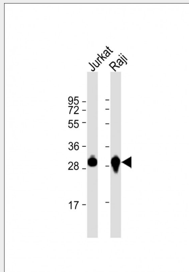
All lanes : Anti-ANP32A Antibody (C-term) at 1:1000 dilution Lane 1: Jurkat whole cell lysate Lane 2: Raji whole cell lysate Lysates/proteins at 20 µg per lane. Secondary Goat Anti-Rabbit IgG, (H+L), Peroxidase conjugated at 1/10000 dilution. Predicted band size : 29 kDa Blocking/Dilution buffer: 5% NFDM/TBST.
