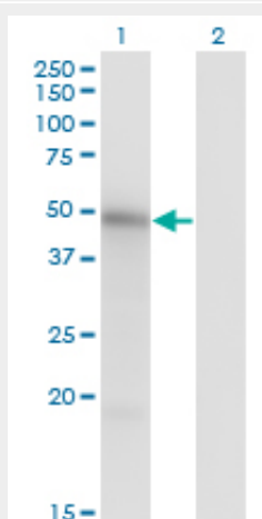
Western Blot analysis of MKNK1 expression in transfected 293T cell line by MKNK1 monoclonal antibody (M08), clone 2H8.
