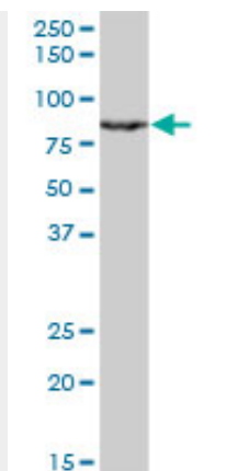
RACGAP1 monoclonal antibody (M01), clone 1G6. Western Blot analysis of RACGAP1 expression in Jurkat (Cat # AT3542a)
