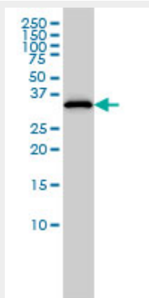
RLBP1 monoclonal antibody (M02), clone 4H5 Western Blot analysis of RLBP1 expression in HepG2 ( Cat # AT3650a )
