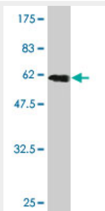
Antibody Reactive Against Recombinant Protein. Western Blot detection against Immunogen (60.61 KDa) .
