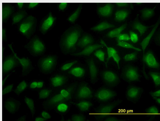
Immunofluorescence of monoclonal antibody to RLBP1 on HeLa cell. [antibody concentration 20 ug/ml]
